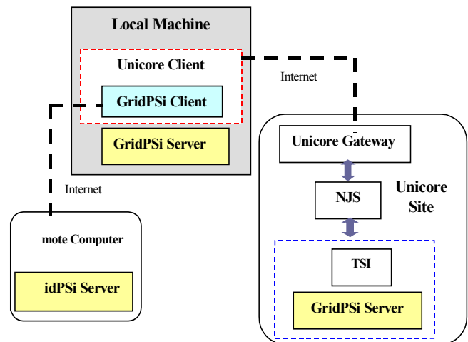
Figure1: GridPSi System Architecture
