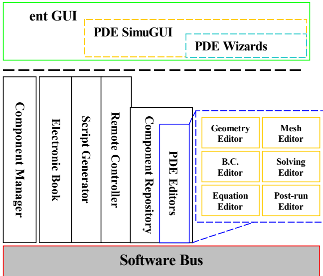
Figure2: GridPSi Client Architecture
