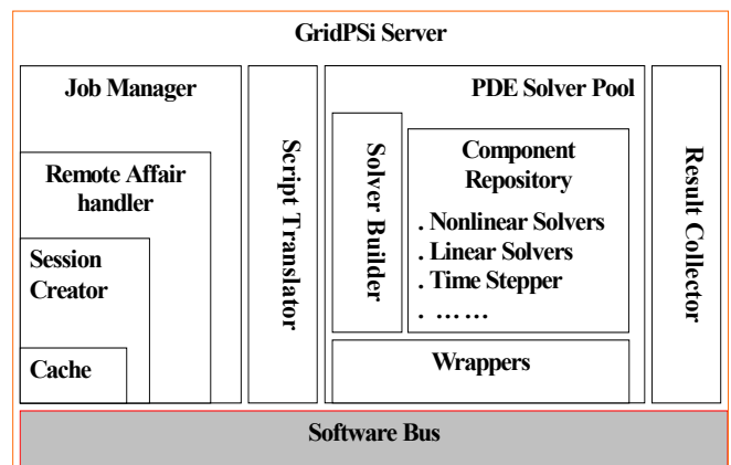
Figure3: GridPSi Server Architecture
